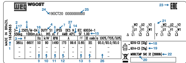
Figure 5 - Nameplate layout for frames 160 to 355
